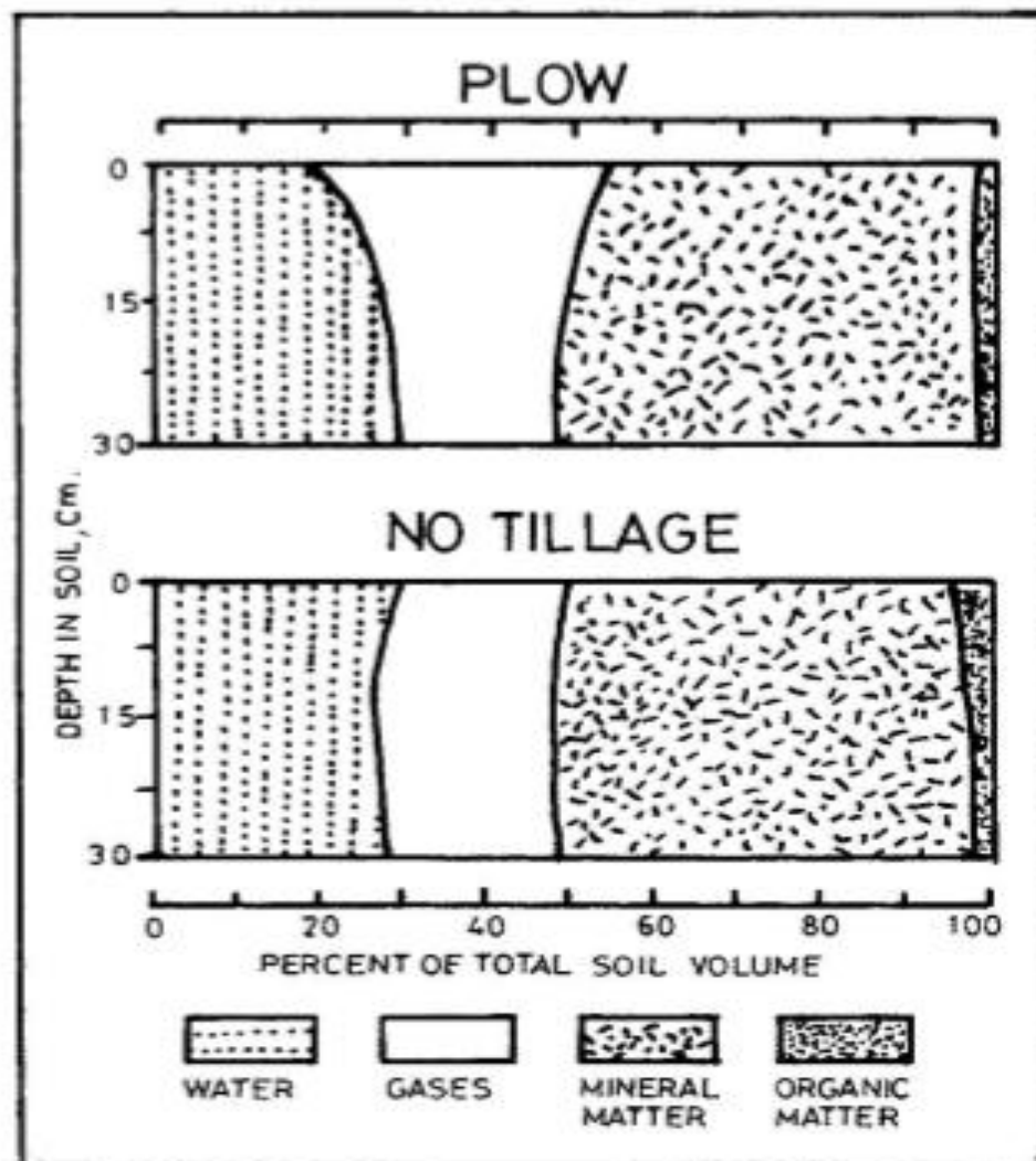
Figure 3.2A. Volume composition of soil when plant growth is in good condition. Tillage increased oxygen concentration in surface (7–8 cm) soil layer. (From Doran, 1982. Crops and Soils Magazine 34:10–12. With permission of ASA.)
