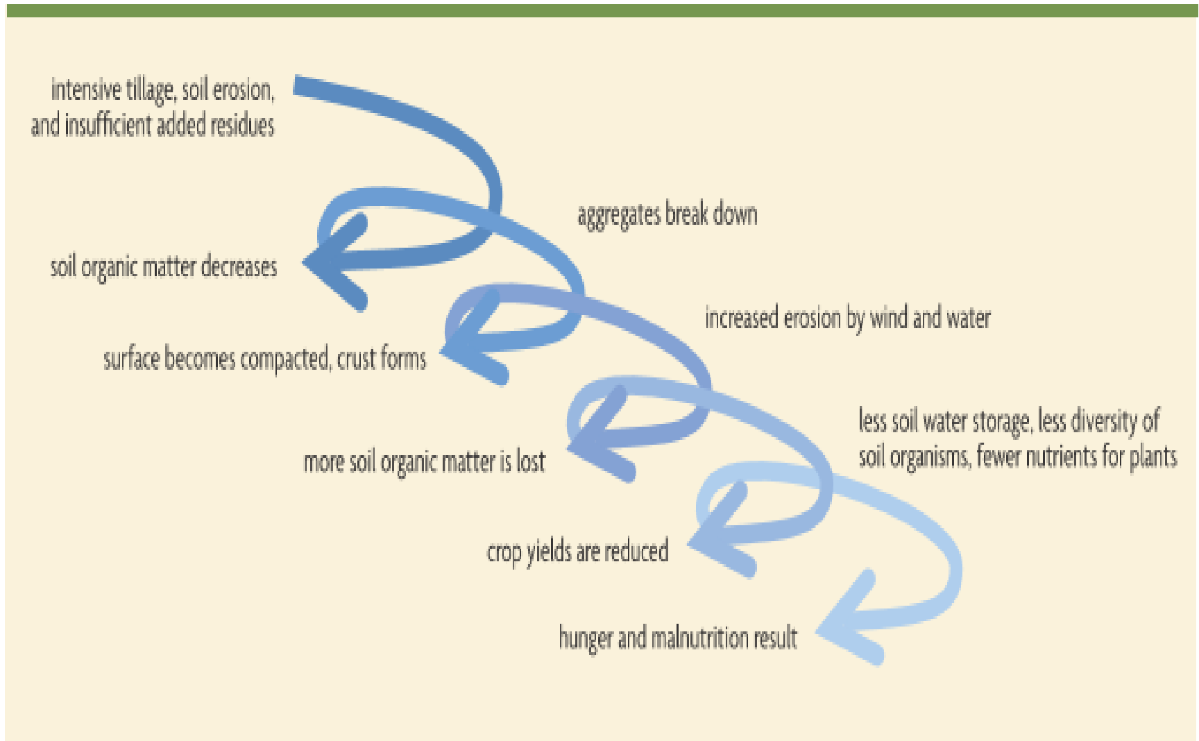
Figure 1.1. The downward spiral of soil degradation. Modified from Topp et al. (1995).
